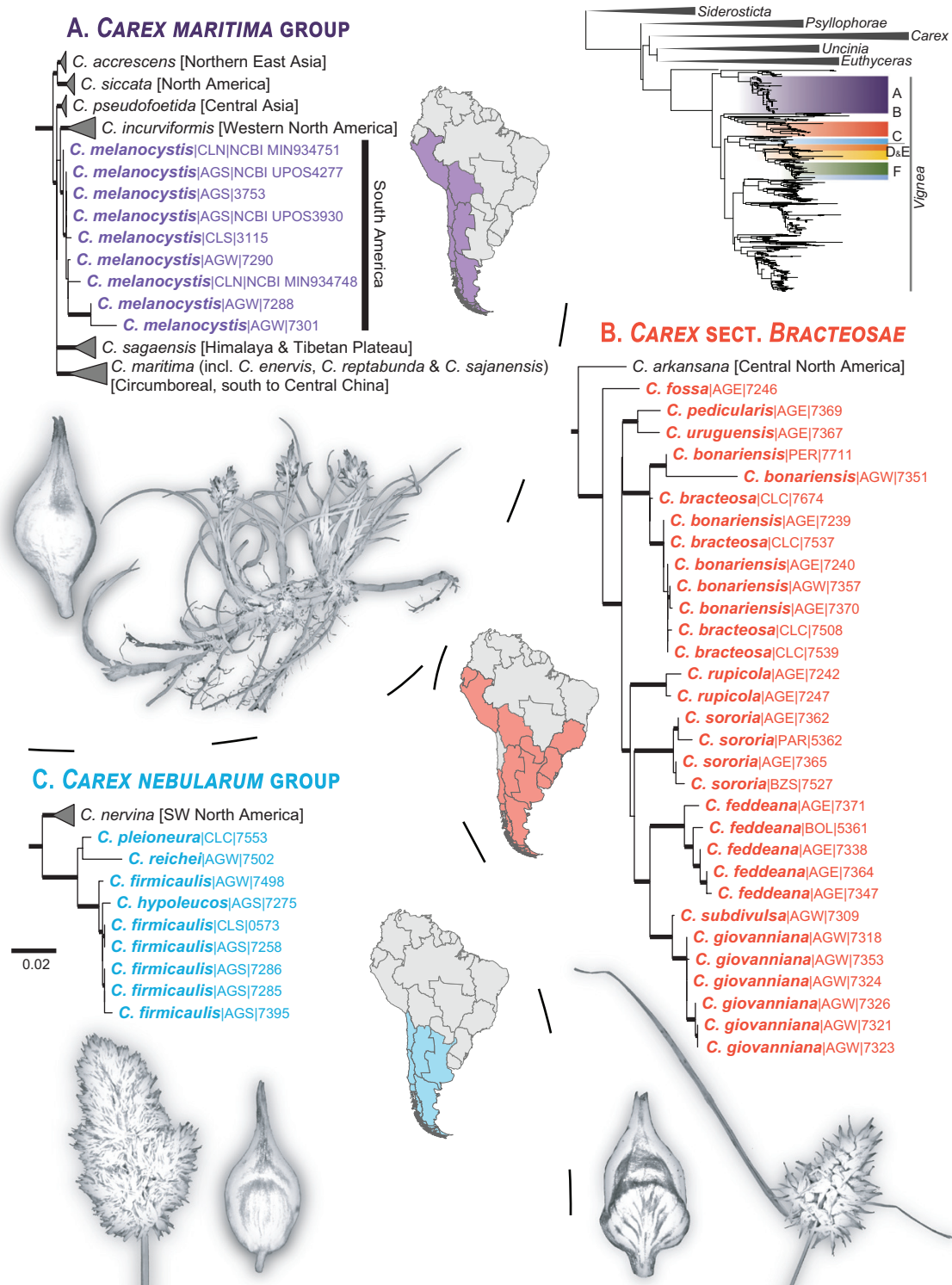
Figure 4. Representative ETS-ITS-matK maximum likelihood (ML) Carex phylogenetic tree with a focus on Carex subgenus Vigna shown in the right corner. The clades including the Neotropical species studied (A-F) are highlighted in different colours. Bold thick branch lines represent non-parametric bootstrapping (BS) clade support > 75%. The labeling of the accessions includes species name, TDWG geographical code and accession number according to Martín-Bravo et al. (2019) . The distribution areas of the species group, section or alliance are shown in coloured maps according to TDWG regions ( Brummitt, 2001 ). Representative image sketches (not to scale) of both inflorescence and utricle of the species are depicted.
